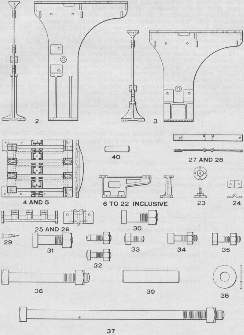
LEGS, TOP PLATES, BOTTOM RAILS, ETC., FOR SAXBY AND FARMER INTERLOCKING MACHINES
